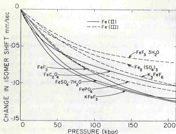
Figure 2. Change of isomer shift vs. pressure diagram for "ionic" compounds.
